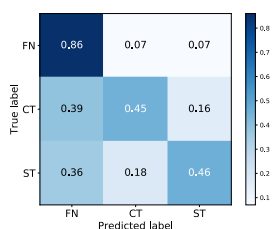
Figure 1: Confusion matrix for categorizing client codes, normalized by row.
